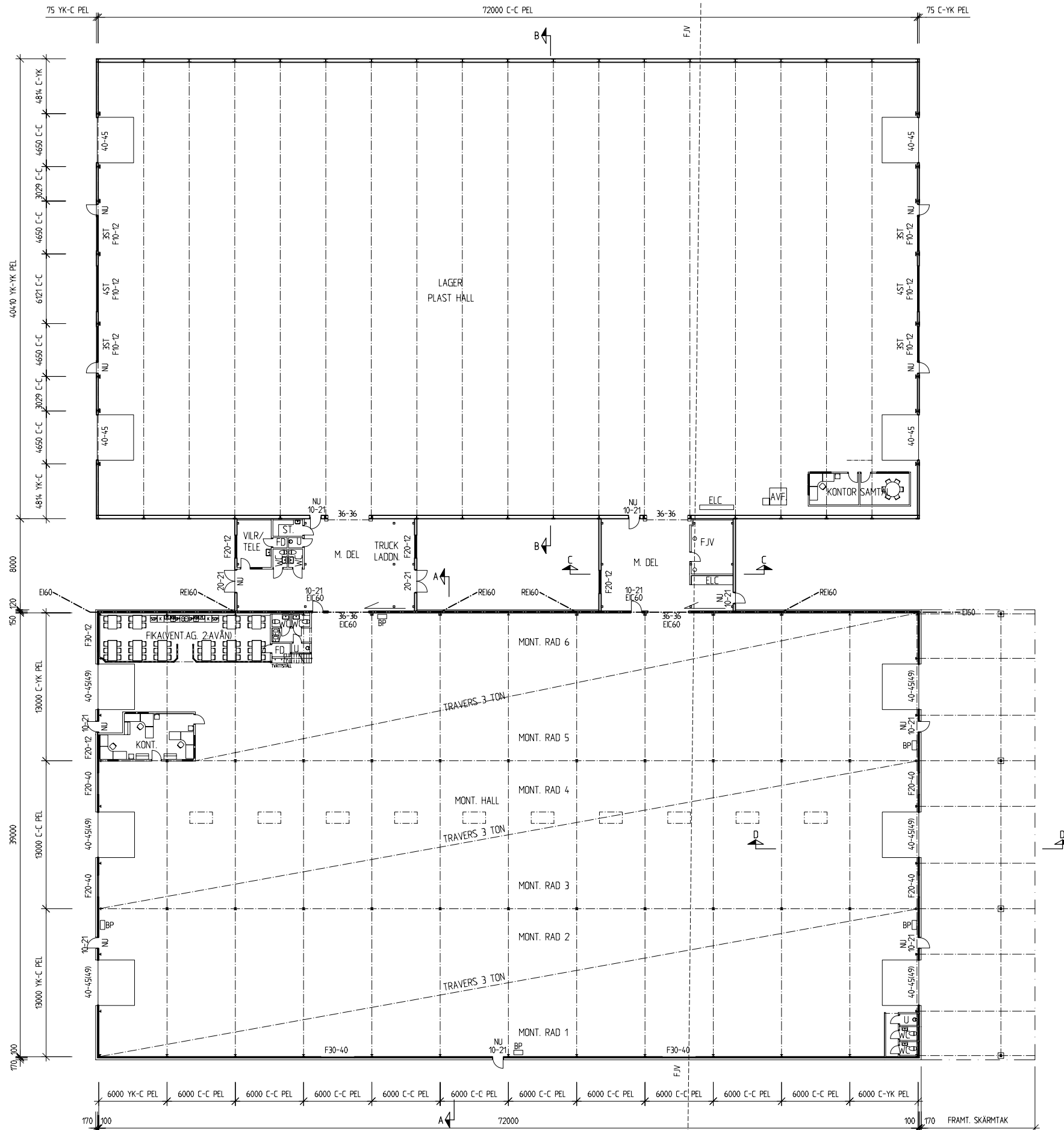
PLAN 1:200
